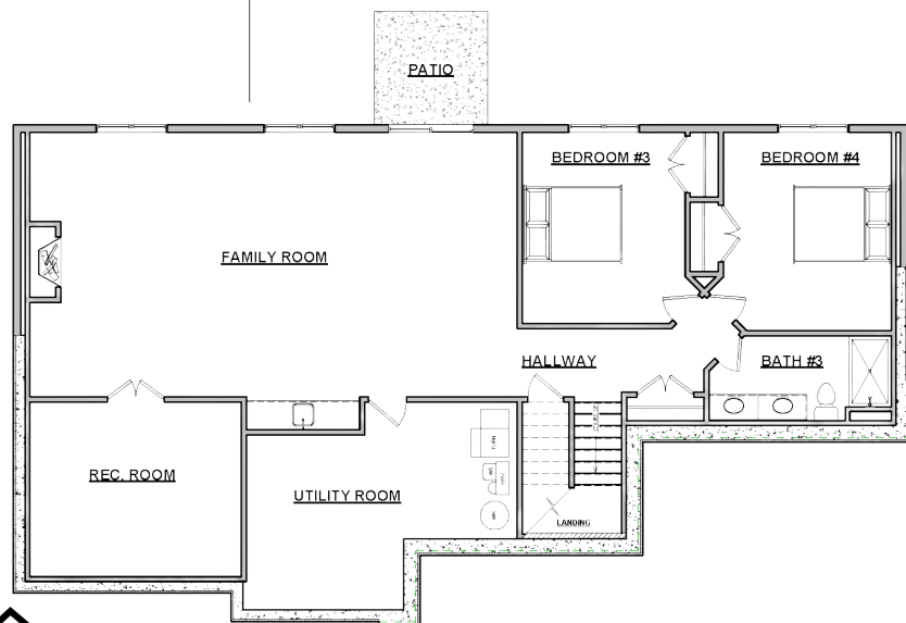
Walkout Basement Floor Plan
