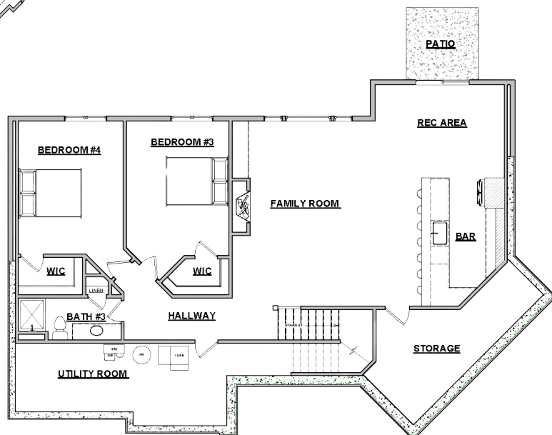
Walkout Basement Floor Plan
