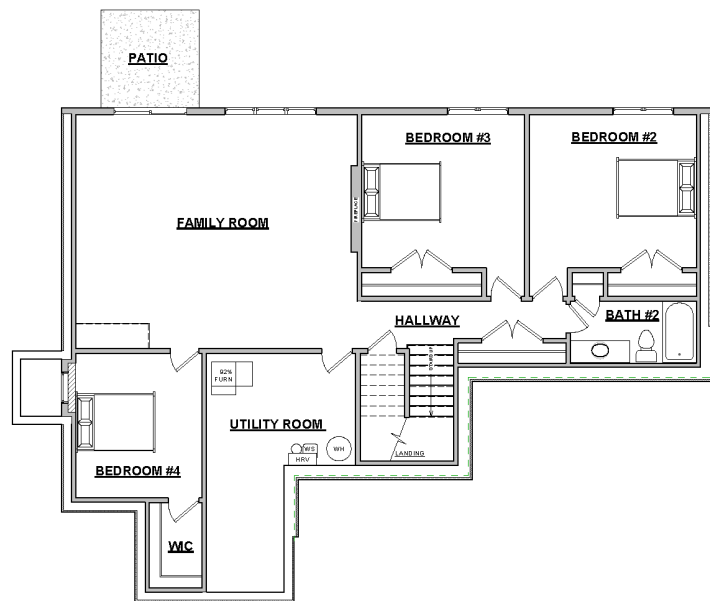
Walkout Basement Floor Plan
